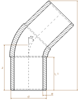
ENJEKSİYON 45 ° DİRSEK INJECTION 45 ° ELBOW PE100 - SDR 17 - PN10 ve SDR 11 - PN16
